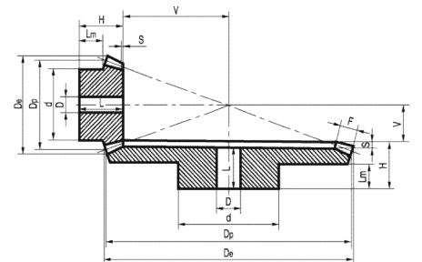
Type B Pressure angle 20° Ratio 1:4
