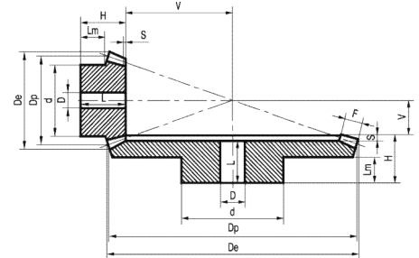
Type B Pressure angle 20° Ratio 1:3
