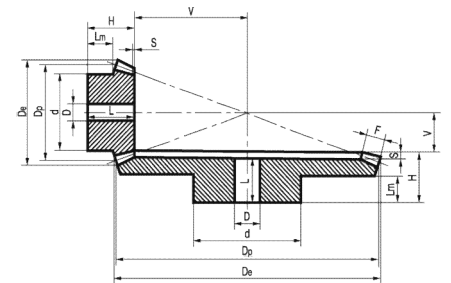
Type B Pressure angle 20° Ratio 1:4
